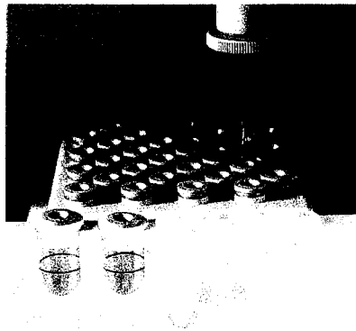
Figure 4. Electropherogram readout of a sequencing reaction. Bottom plate illustrates capillary 310 platform.
