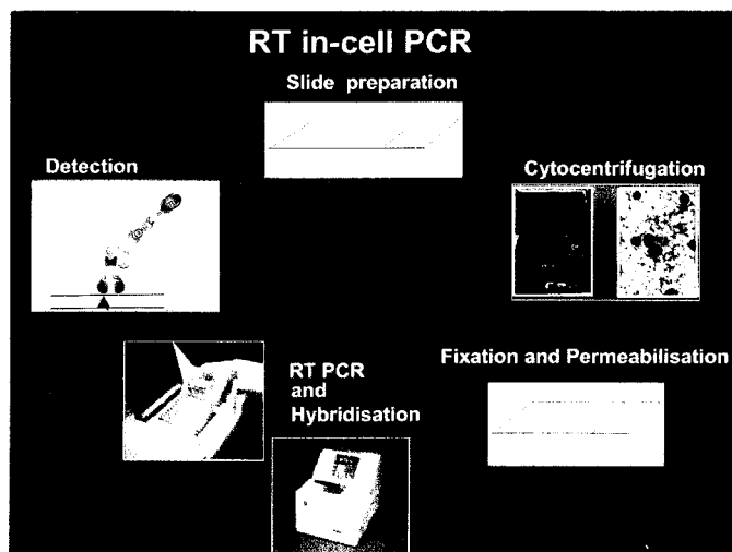
Figure 1: Schematic representation of RT in-cell PCR
