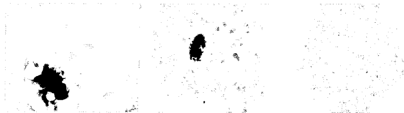
Figure 6 (above) demonstrates in-cell PCR results in patients with SSPE. Note the presence of measles virus genomes in brain tissue of affected patients.
