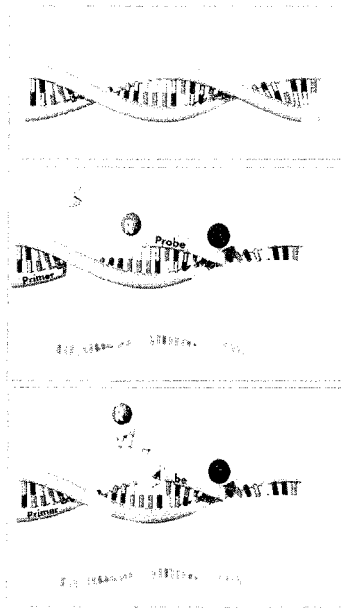
Figure 3 Schematic representation of TaqMan PCR
