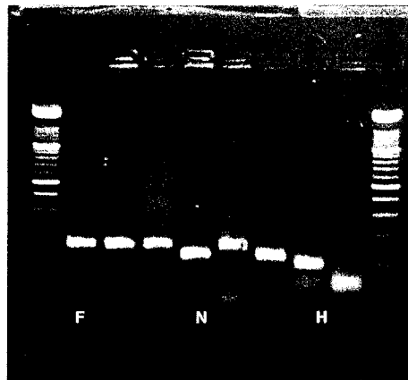
Figure 2 Solution phase PCR of F,N and H genes of measles virus.
