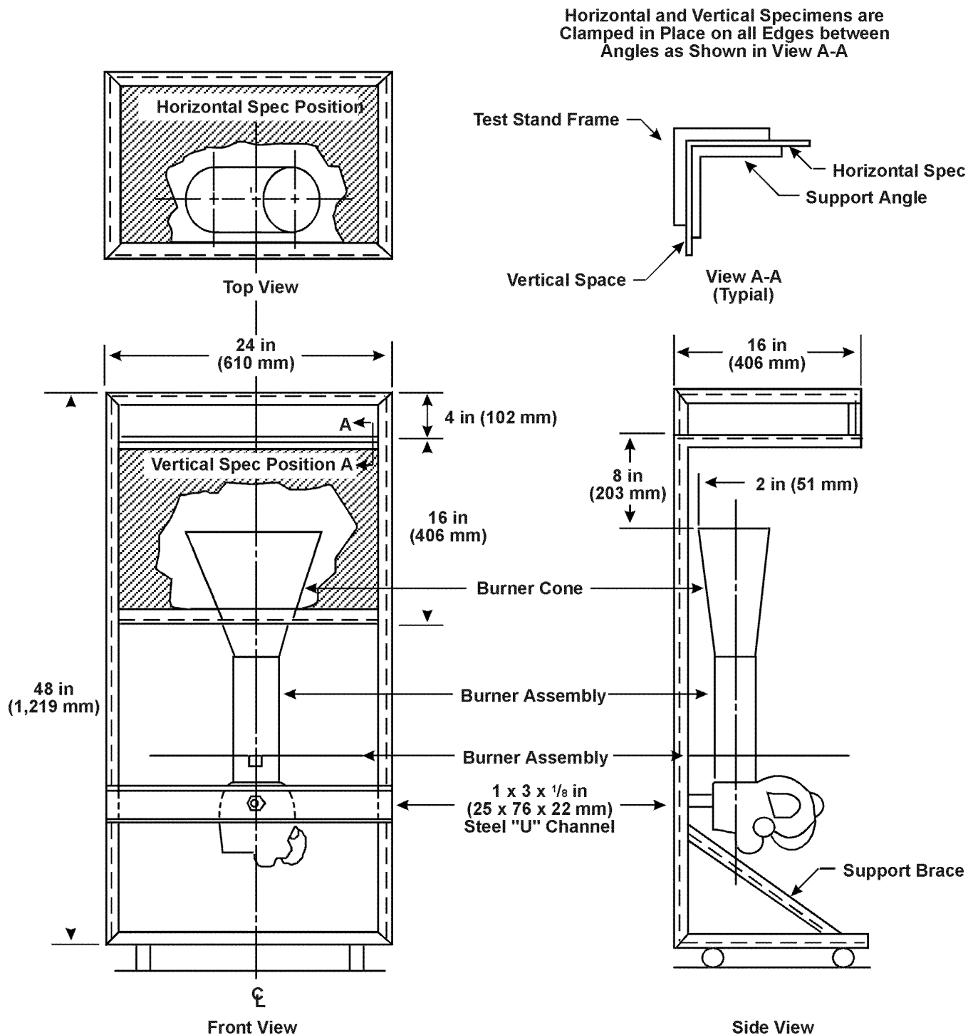
Figure 1: Test Apparatus for Horizontal and Vertical Mounting
