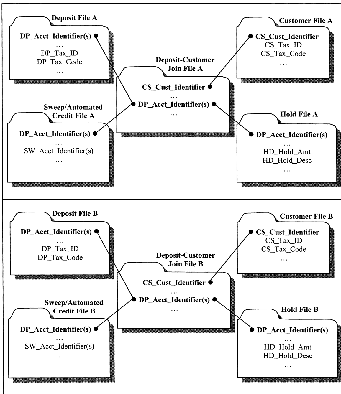
Figure 3. Multiple File Sets.
